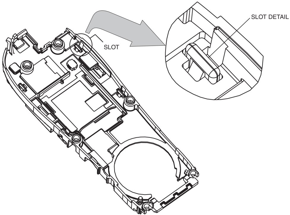
Figure 11 Display Removal - Holders Release
