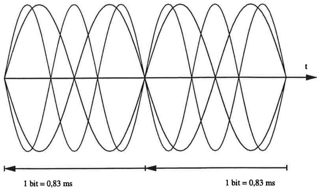
Fig. 4.6.3 Line diagram for the FFSK signal
