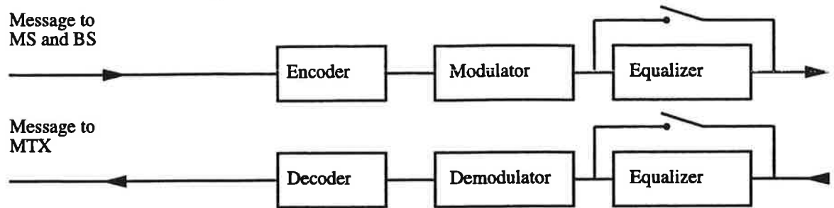
Fig. 4.6.1 Functional block diagram of the 1200 Baud signalling equipment at MTX
