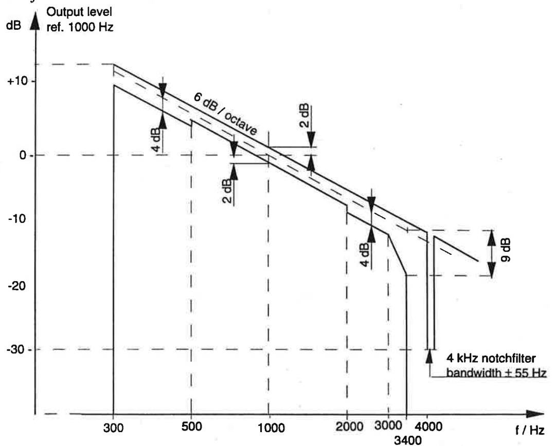
Figure 3. Audio frequency response of the combination receiver line interface
