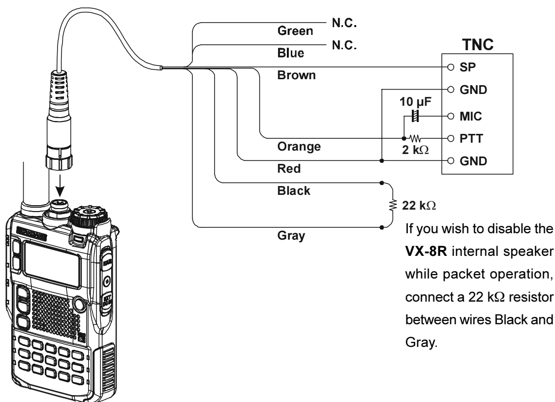
CT-M11 MIC/SP Connection Cable
